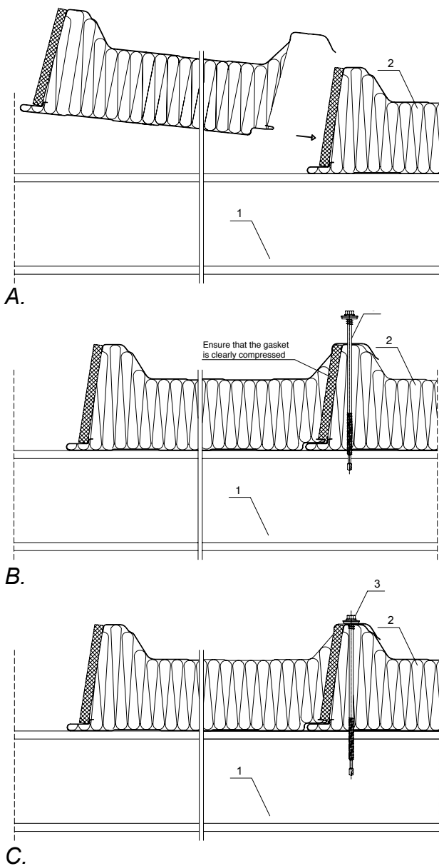
Fig. 19. Sample assembly of sandwich panels, where: 1 – beam 2 – sandwich panel SP2C PIR 3 – fastener
