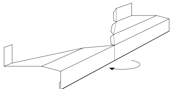
Fig.19. Plinth flashing external corner.
